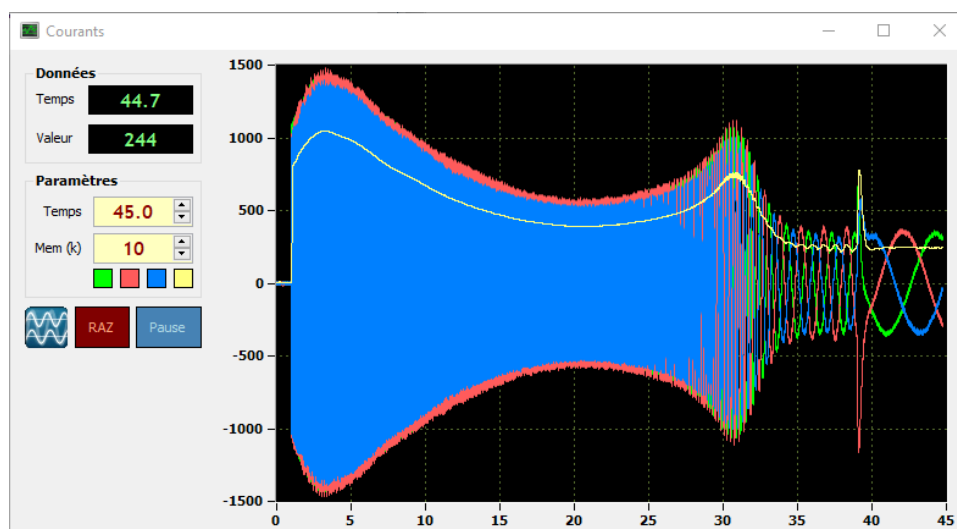
AKAMAS rotor current plot
