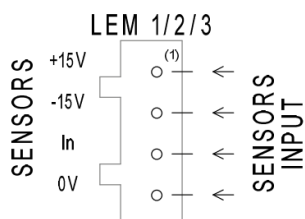
Connectors CT1, CT2, CT3 and CT4: Current sensors
