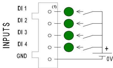
Connector C3: Logic inputs AoN
